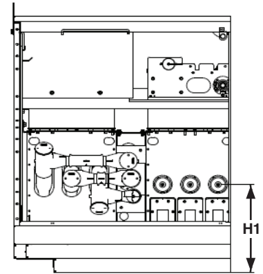
TYPICAL CABLE INTERFACE VIEW FOR SWITCHES AND FAULT INTERRUPTERS
