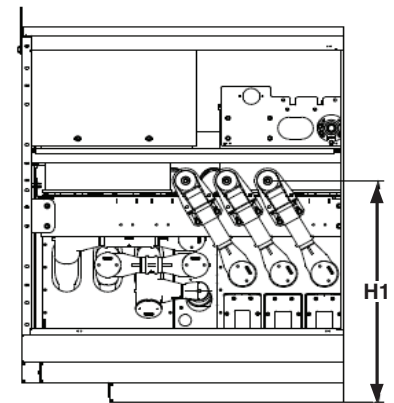
Typical Cable Interface View For Switches with Cable Centerline Adapters
