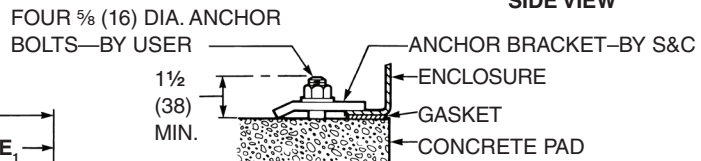
ANCHOR BOLT DETAIL
