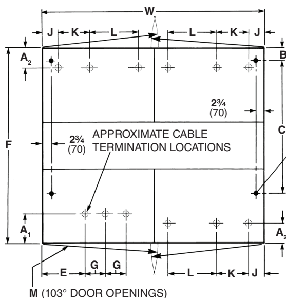
ANCHOR BOLT PLAN
