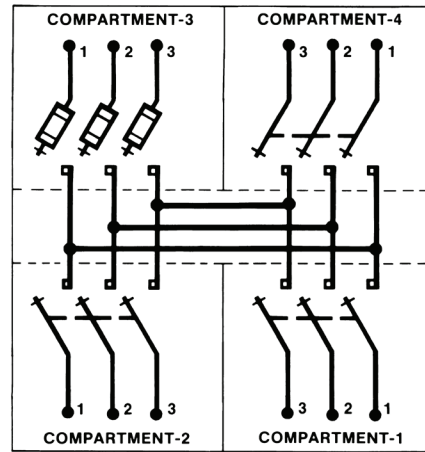
CONNECTION DIAGRAM
