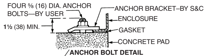
ANCHOR BOLT DETAIL
