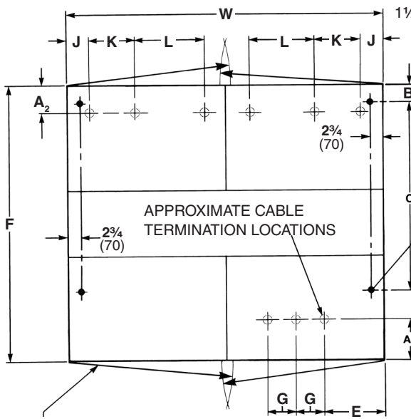
ANCHOR BOLT PLAN
