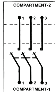
CONNECTION DIAGRAM
