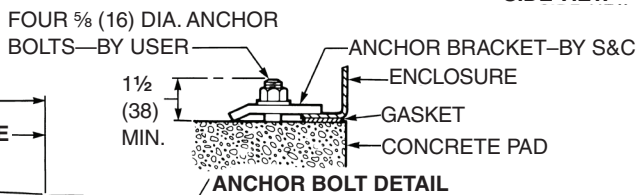
ANCHOR BOLT DETAIL
