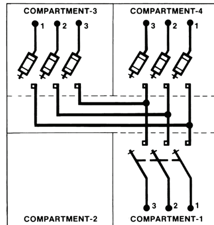
CONNECTION DIAGRAM
