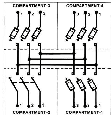
CONNECTION DIAGRAM
