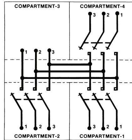
CONNECTION DIAGRAM
