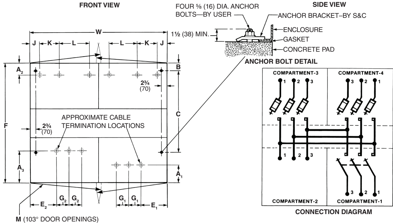
ANCHOR BOLT PLAN
