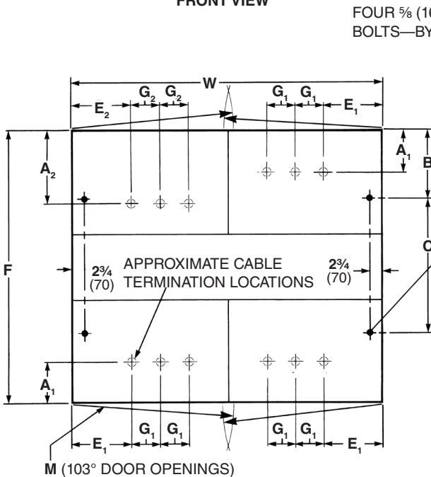
ANCHOR BOLT PLAN
