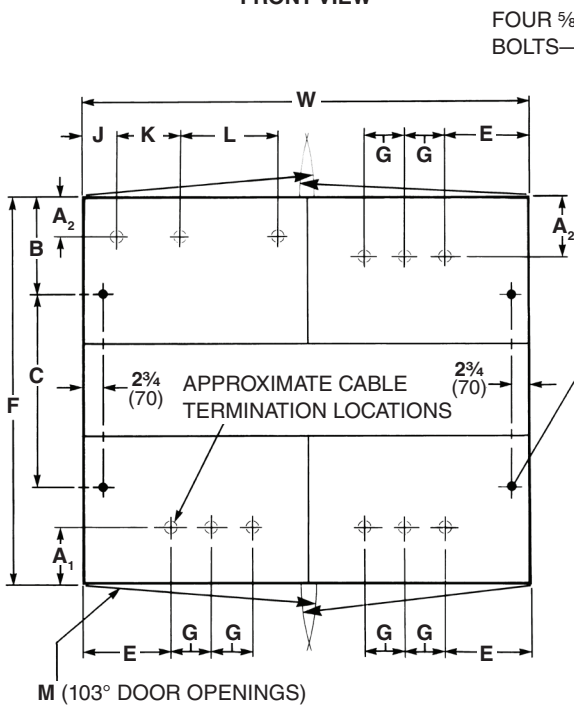
ANCHOR BOLT PLAN
