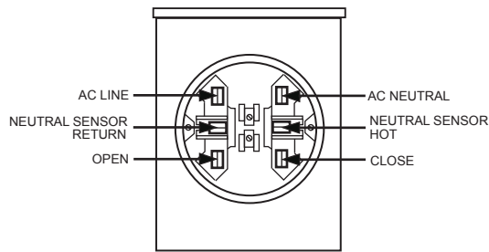
Six-Jaw Electric Meter Base, Catalog Number Suffix "-J68"
