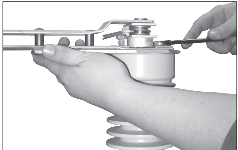
Figure 14. Loosen the blade hardware if necessary and move blade to the fully-closed position against the bumper stop.
