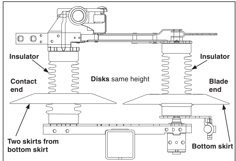
Figure 9. Wildlife disk placement on 25-kV Omni-Rupter Switches.
