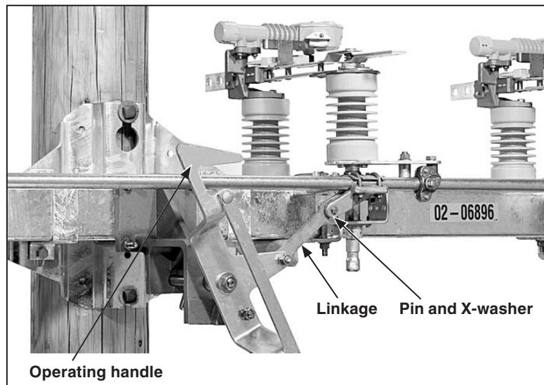
Figure 2. Install pin and X-washer to connect linkage.
