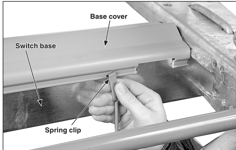
Figure 6. Hook one end of spring clip into base cover lip. Stretch underneath base and hook on opposite side.
