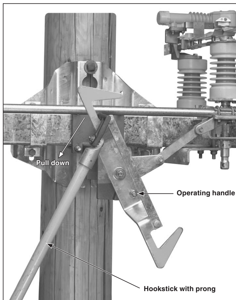
Figure 20. Firmly pull operating handle with hookstick.
