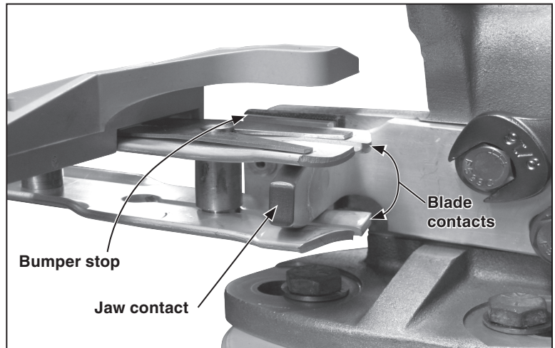
Figure 13. Make sure the jaw contact is fully-centered between the blade contacts and that the blade contacts are against the bumper stop.
