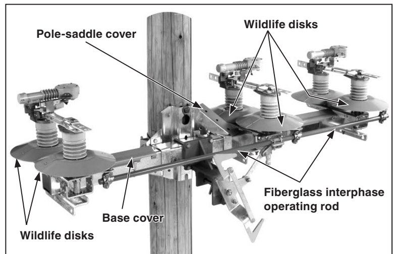
Figure 5. 14.4-kV Omni-Rupter with Optional Wildlife Protection (Catalog Number Suffix “-W”), Upright Mounting Configuration.
