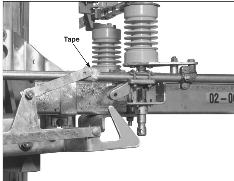
Figure 1. Removal of tape securing the operating linkage.
