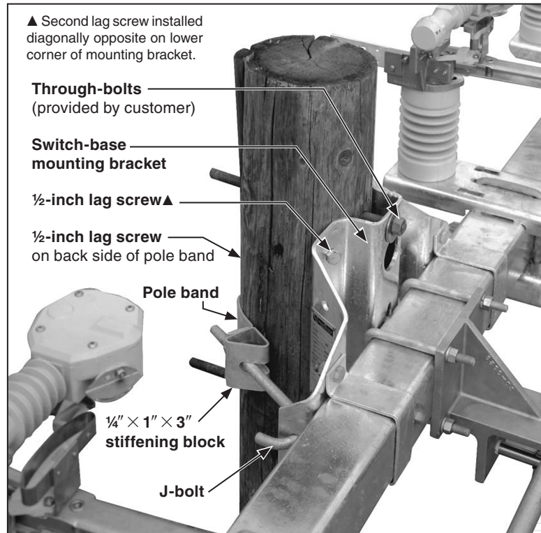
Figure 4. Typical pole-band attachment detail.
