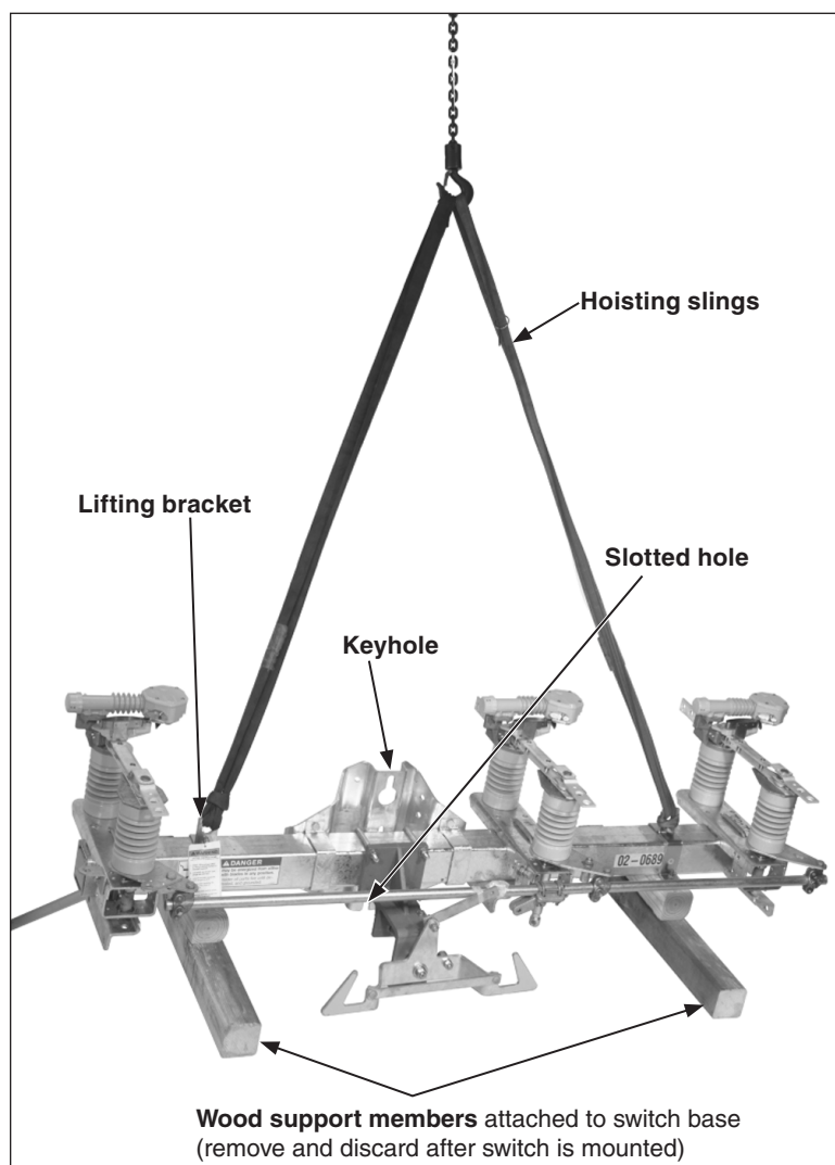
Figure 3. Hoisting the Omni-Rupter Switch into position.
