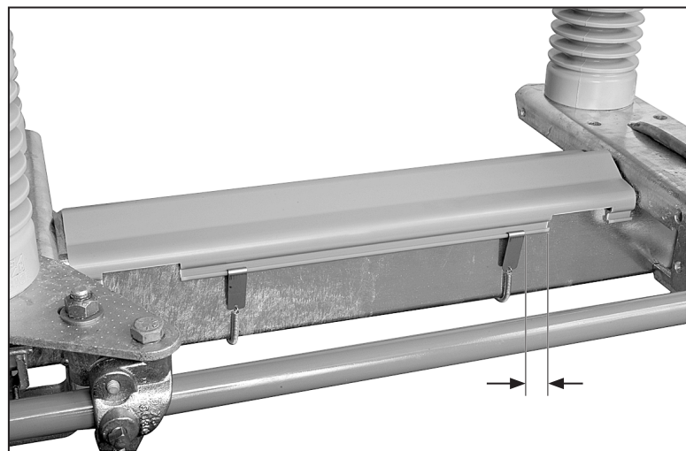
Figure 7. Make sure clips are installed 1/2-inch from edge of cover.
