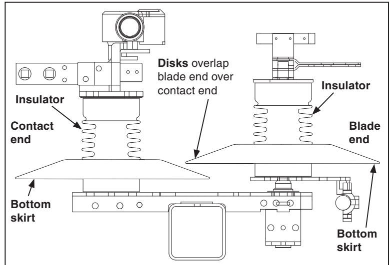
Figure 8. Wildlife disk placement on 14.4-kV Omni-Rupter Switches.
