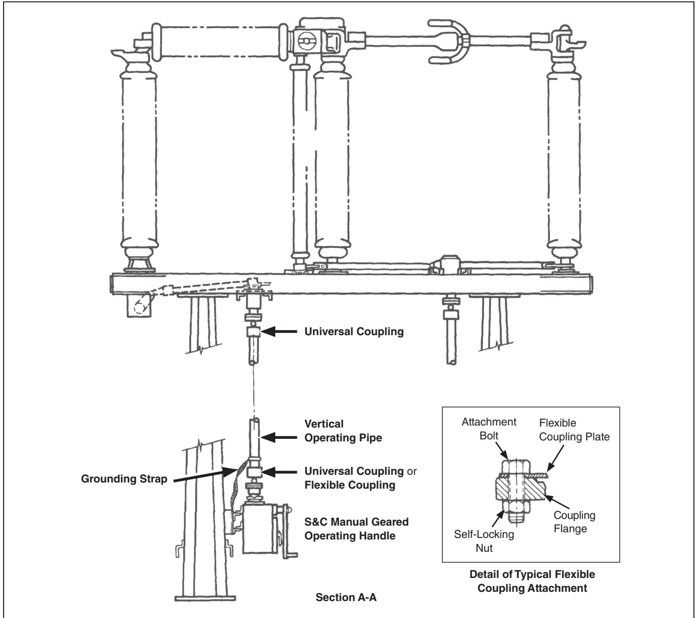
Figure 3. Detail view of installation of S&C Manual Geared Operating Handle.
