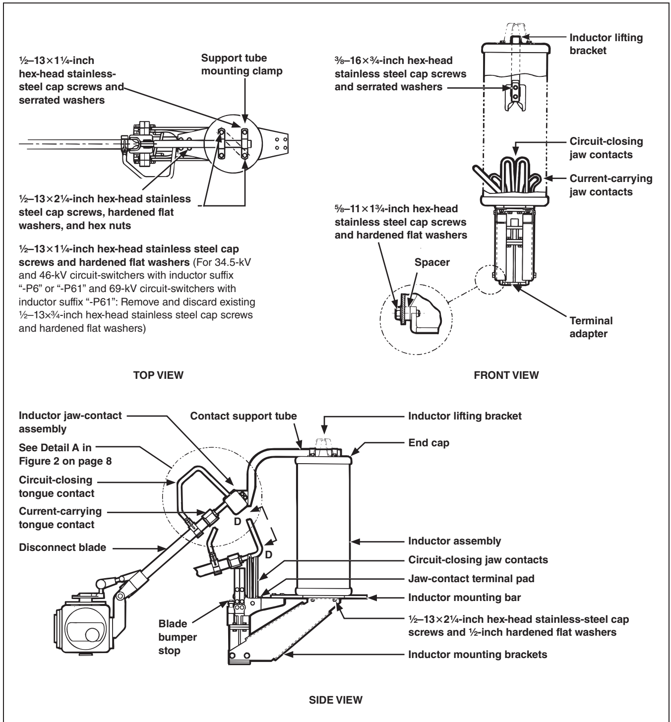
Figure 1. Top, front, and side view assembly details of standard-duty pre-insertion inductors for 34.5-kV through 69-kV vertical-break style and integer-style circuit-switchers.
