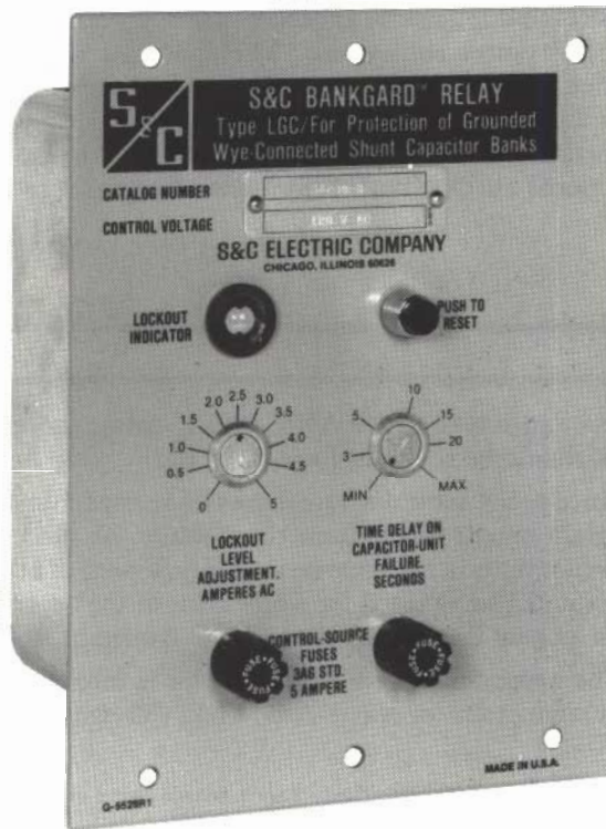
Figure 1. S&C Bankgard Relay—Type LGC.
