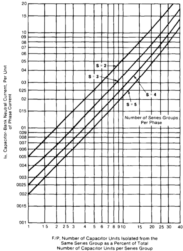
Figure 5. Per-unit capacitor-bank neutral current versus percentage of capacitor units isolated from the same series group.
