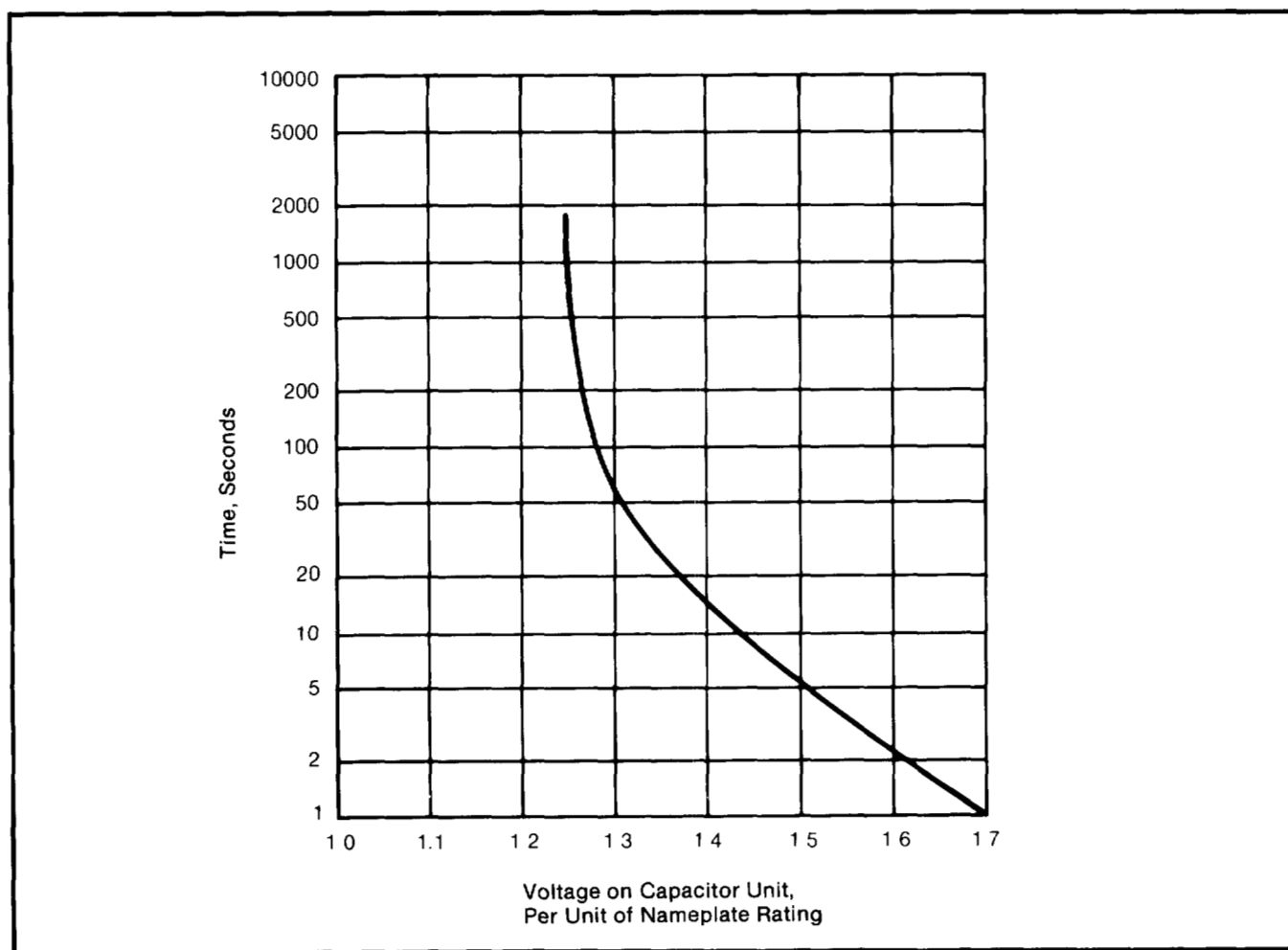
Figure 2. Capacitor-unit power-frequency overvoltage versus time, as permitted by ANSI/IEEE Standard 18-1980, "IEEE Standard for Shunt Power Capacitors," which further states that capacitors shall be capable of continuous operation up to 110% of rated voltage, including harmonics. Note: This curve applies for up to 300 applications of power-frequency overvoltages of the magnitudes and durations illustrated. Capacitor manufacturers may publish different recommendations applicable to their particular units.
