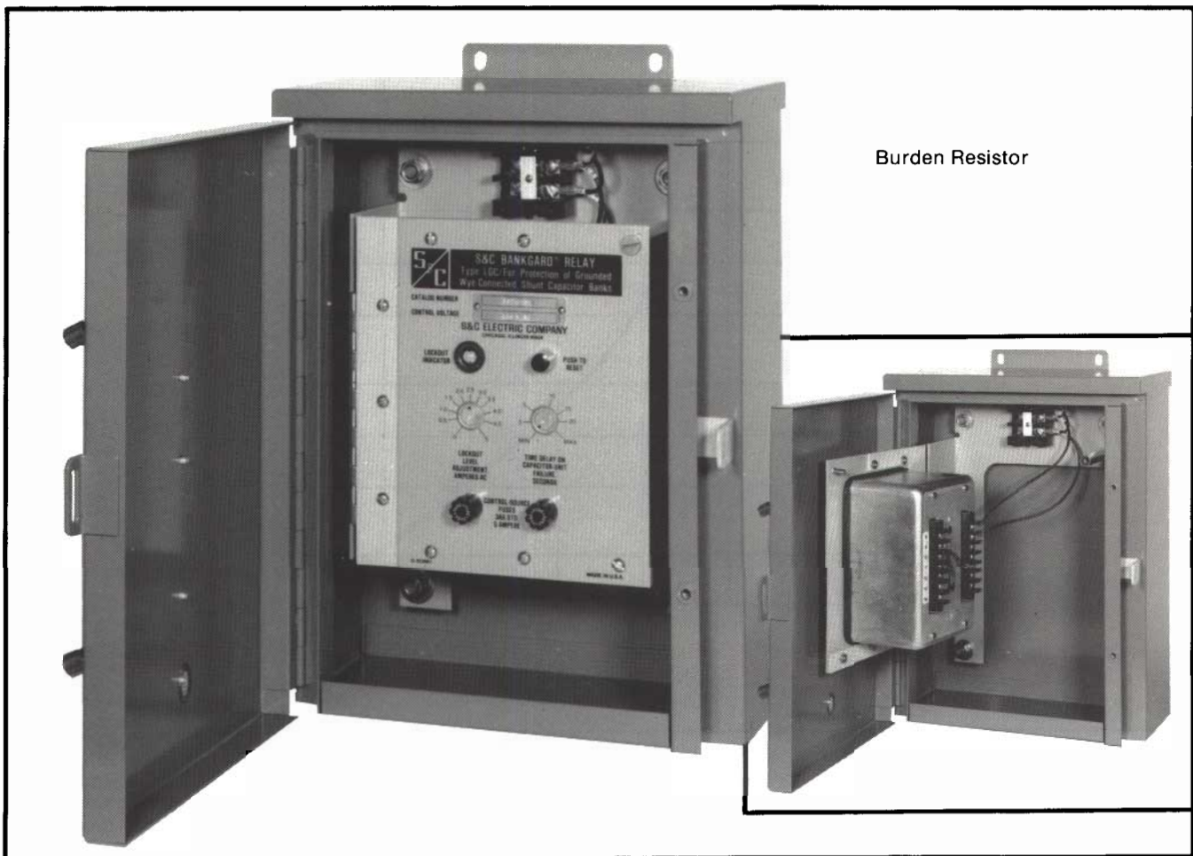
Figure 3. S&C Type LGC Bankgard Relay mounted in the accessory weatherproof steel enclosure. Relay is hinge-mounted to facilitate access to the terminal blocks.
