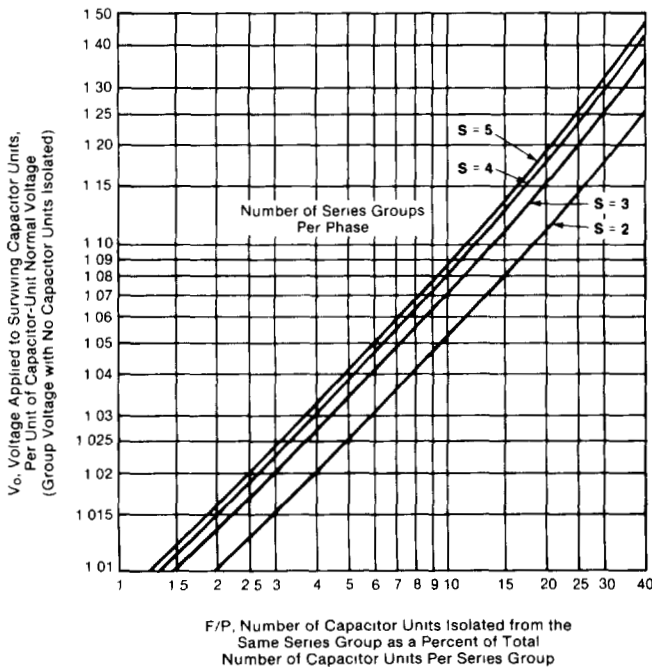
Figure 4. Per-unit voltage applied to surviving capacitor units in a series group versus percentage of capacitor units isolated from the same series group.
