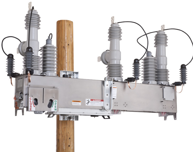
38-kV IntelliRupter PulseCloser Fault Interrupter featuring IntelliTeam II software.
