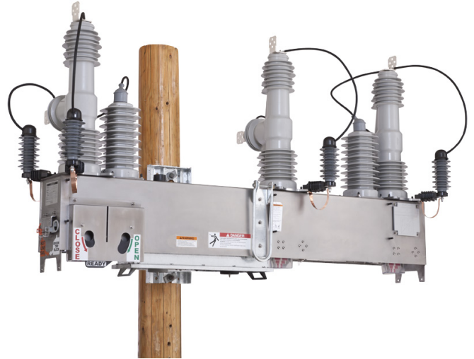
S&C IntelliRupter PulseCloser Fault Interrupter.
